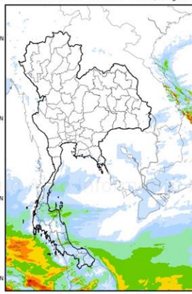
WRF-ROMS (ThaiGeo), 24-Hour Precipitation, Thailand Model (3x3 km) 26-Nov-2017 19:00 to 27-Nov-2017 19:00 (Bangkok Time)
