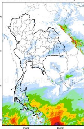
WRF-ROMS (ThaiGeo), 24-Hour Precipitation, Thailand Model (3x3 km) 28-Nov-2017 19:00 to 29-Nov-2017 19:00 (Bangkok Time)
