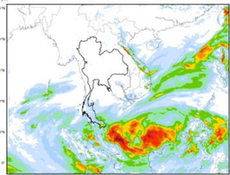
WRF-ROMS (ThaiGeo), 24-Hour Precipitation, Southeast Asia Model (9x9 km) 30-Nov-2017 19:00 to 01-Dec-2017 19:00 (Bangkok Time)
