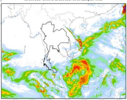
WRF-ROMS (ThaiGeo), 24-Hour Precipitation, Southeast Asia Model (9x9 km) 01-Dec-2017 19:00 to 02-Dec-2017 19:00 (Bangkok Time)
