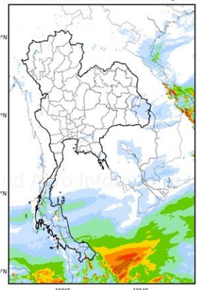
WRF-ROMS (ThaiGeo), 24-Hour Precipitation, Thailand Model (3x3 km) 27-Nov-2017 19:00 to 28-Nov-2017 19:00 (Bangkok Time)
