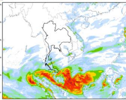
WRF-ROMS (ThaiGeo), 24-Hour Precipitation, Southeast Asia Model (9x9 km) 29-Nov-2017 19:00 to 30-Nov-2017 19:00 (Bangkok Time)
