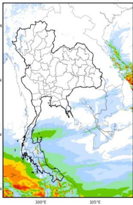
WRF-ROMS (ThaiGeo), 24-Hour Precipitation, Thailand Model (3x3 km) 26-Nov-2017 07:00 to 27-Nov-2017 07:00 (Bangkok Time)
